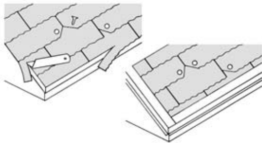
Figure 12-19: Preparing an old roof for reroofing.
