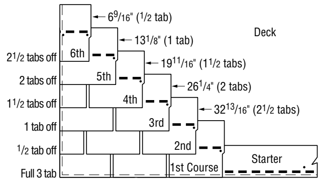
Figure 12-17: Half-Tab Method.
