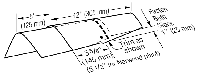
Figure 12-25: Installation of caps along the hips and ridges.
