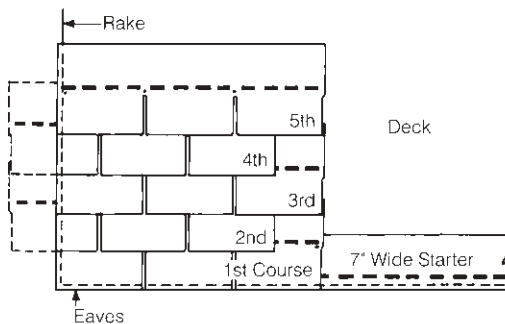
Figure 12-12: Vertical Racking Method.
