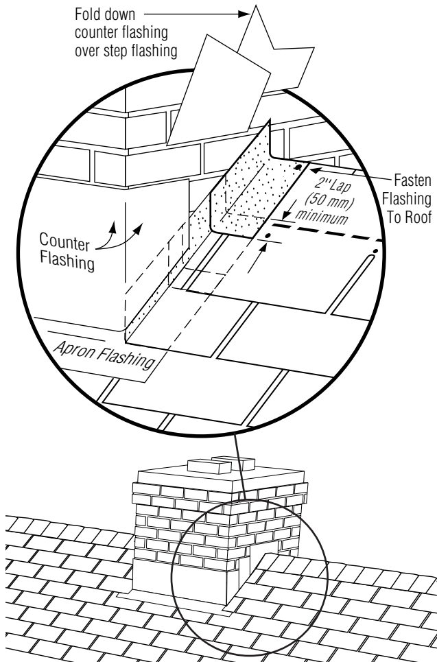
Figure 12-18: Flashing around a chimney.
