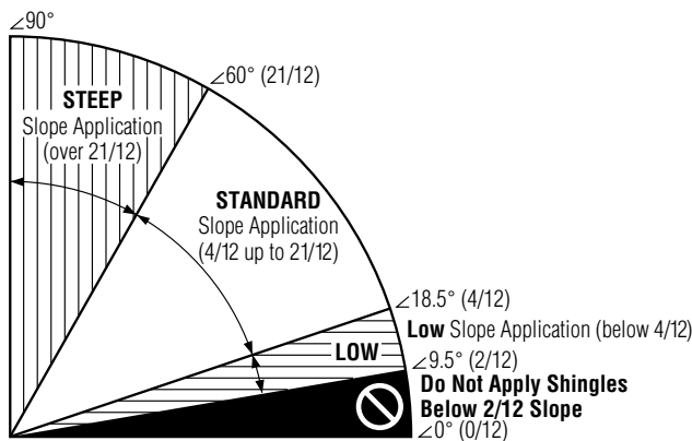
Figure 12-1: Slope definitions.
